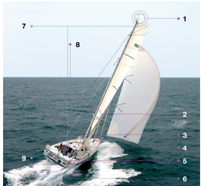
Figure 2. The SolOceans One-design with the indicated positions of the already installed (purple) and future sensors (until 2012, cyan): 1. wind direction and speed, 2. air humidity and temperature and 3. atmospheric pressure. The flow-through system (6.) includes the sensors for sea surface salinity and temperature (4.) as well as sea surface p\text{CO}_2 (5.). In the future it will also host a fluorescence and a pH sensor; the mast top will also be equipped with a radiation measuring device (7.). 8. denotes the satellite transmission of the collected data and 9. marks the position of the hydro generator. Photo: Jean-Marie Liot - SailingOne
