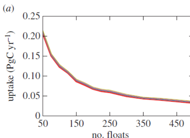
Fig. 7 Error estimate for the annual reconstruction of Southern Ocean CO 2 uptake for varying number of floats. Southern Ocean (beyond 30°S) CO 2 uptake is ~0.8 PgC yr -1 . The fractional error at 200 floats is near 10%. From [Majkut et al. , 2014].
